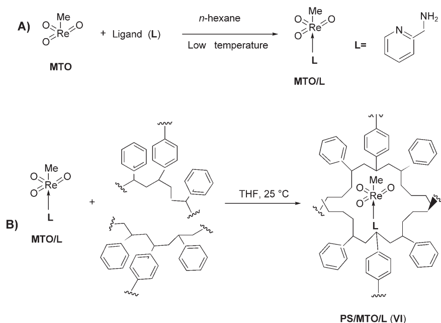
Figure 3. Schematic representation of the PS/MTO/L catalyst ( VI ) prepared by encapsulation with polystyrene of the complex between MTO and 2-aminomethylpyridine ( MTO/L ).
