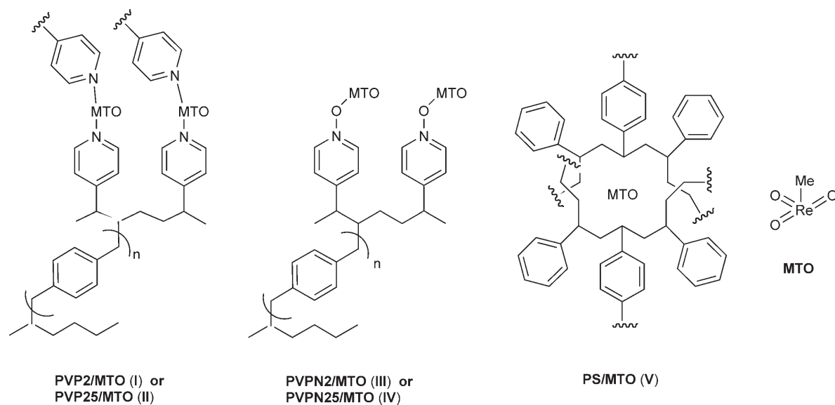
Figure 2. Schematic representation of the structure of poly(4-vinylpyridine), poly(4-vinylpyridine N -oxide), and polystyrene/methylrhenium trioxide (PVP/MTO, PVPN/MTO and PS/MTO, respectively) systems ( I–V ). n = % of divinylbenzene units.
